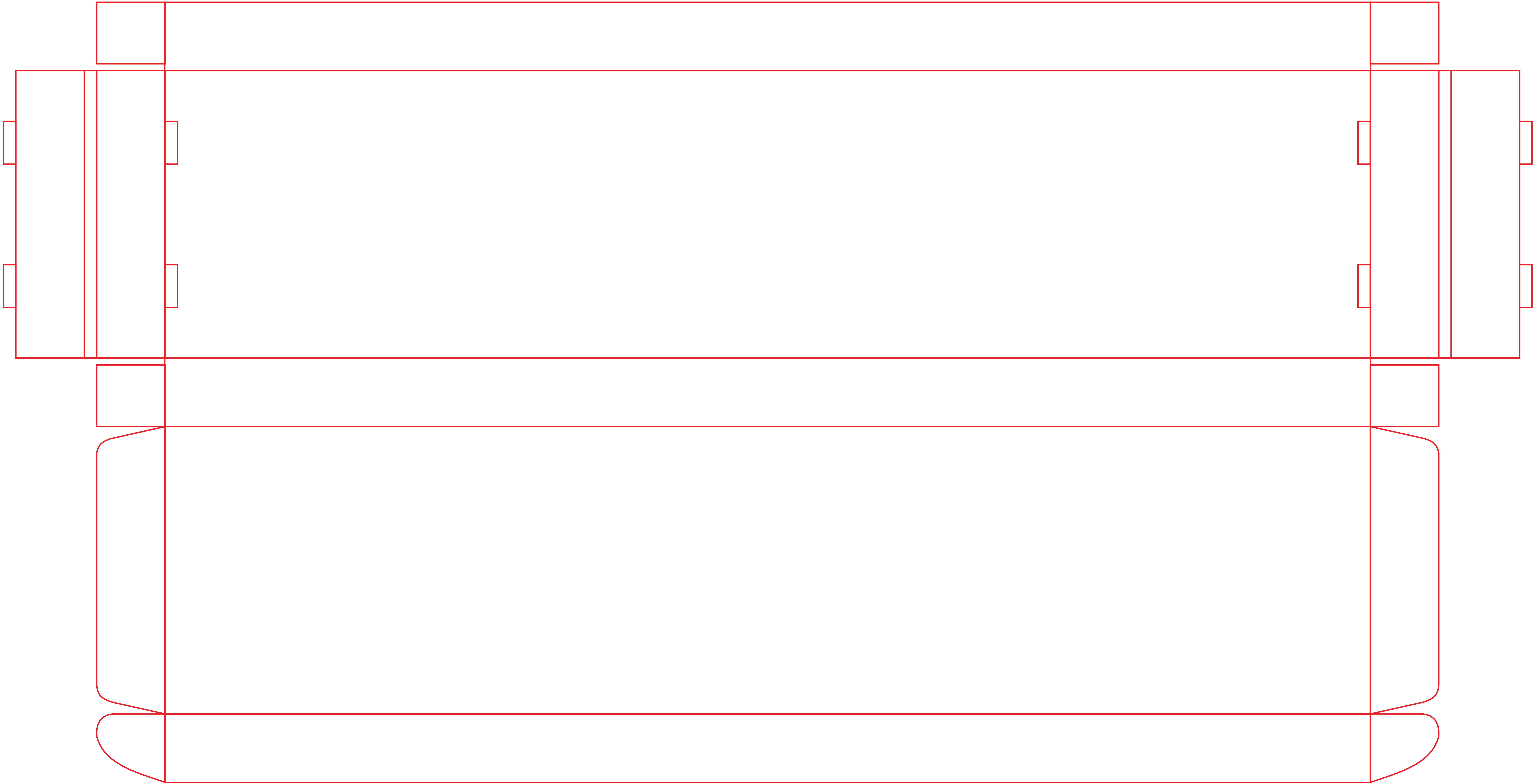
PLB135XL:880x210x50mm
